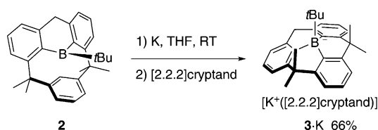
Scheme 3. Reduction of boracyclopentane 2 .
